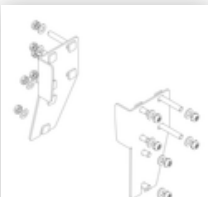
Order no.: 800016 Mounting kit for support section
